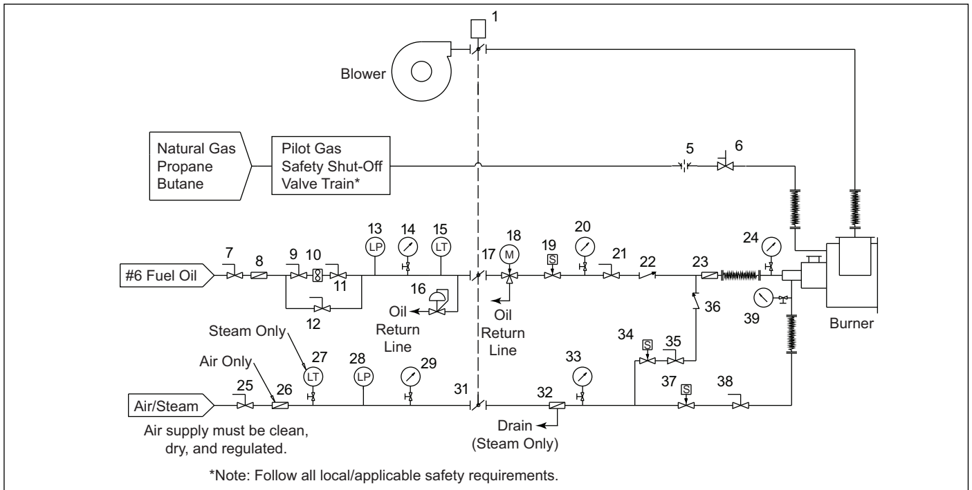
Figure 3.7 - Schematic for #6 Fuel Oil
