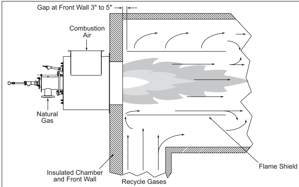
Figure 3.2 - Flame Shield (Typical Example with Gap)
