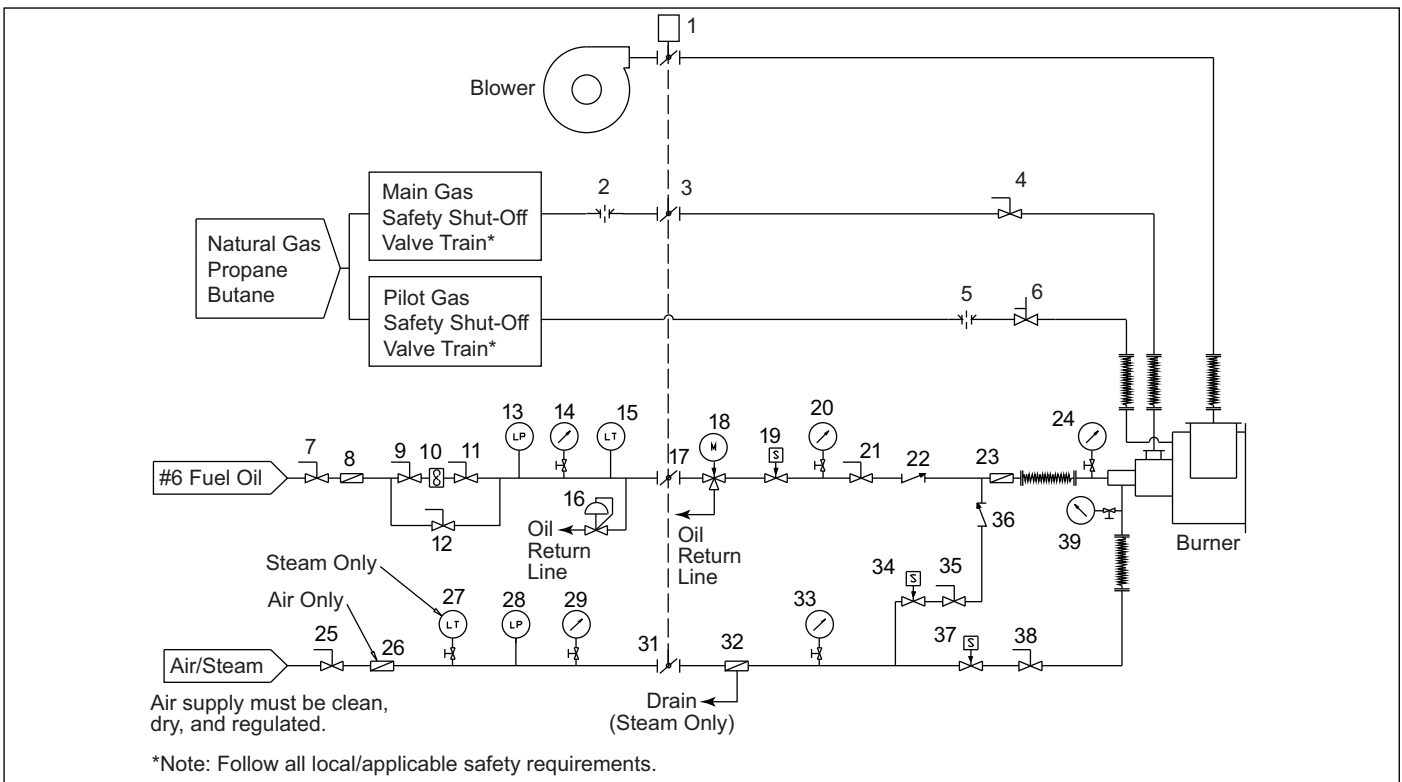
Figure 3.5 - Schematic for Natural Gas, Propane, Butane and #6 Fuel Oil
