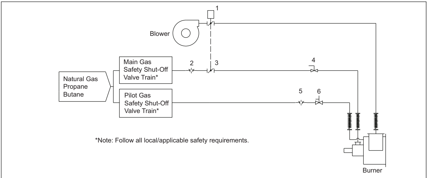
Figure 3.4 - Schematic for Natural Gas, Propane, & Butane
