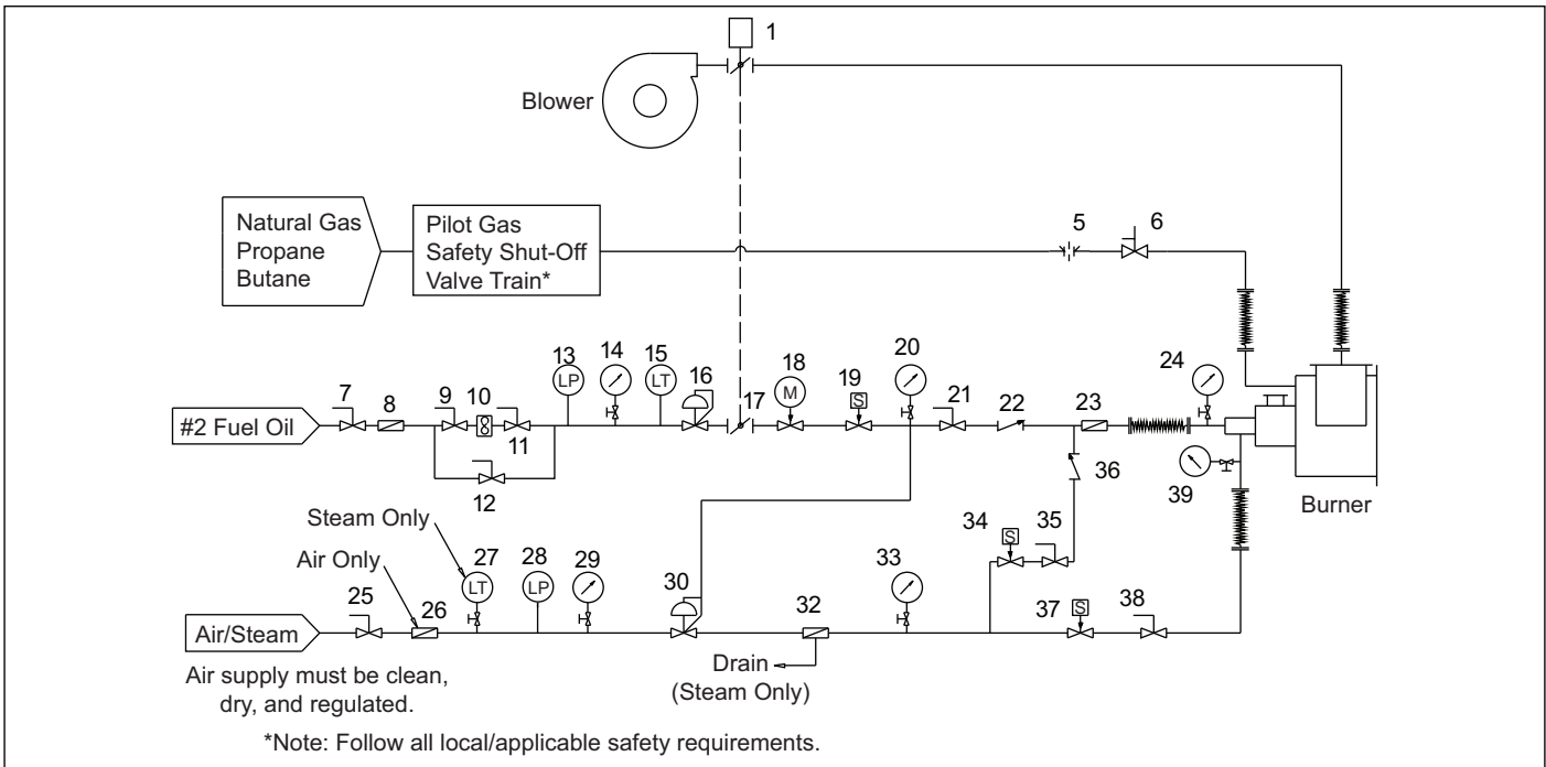
Figure 3.8 - Schematic for #2 Fuel Oil
