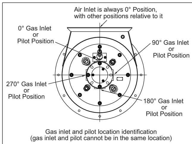
Figure 3.1 - Gas Lance & Gas Pilot (Optional Positions)
