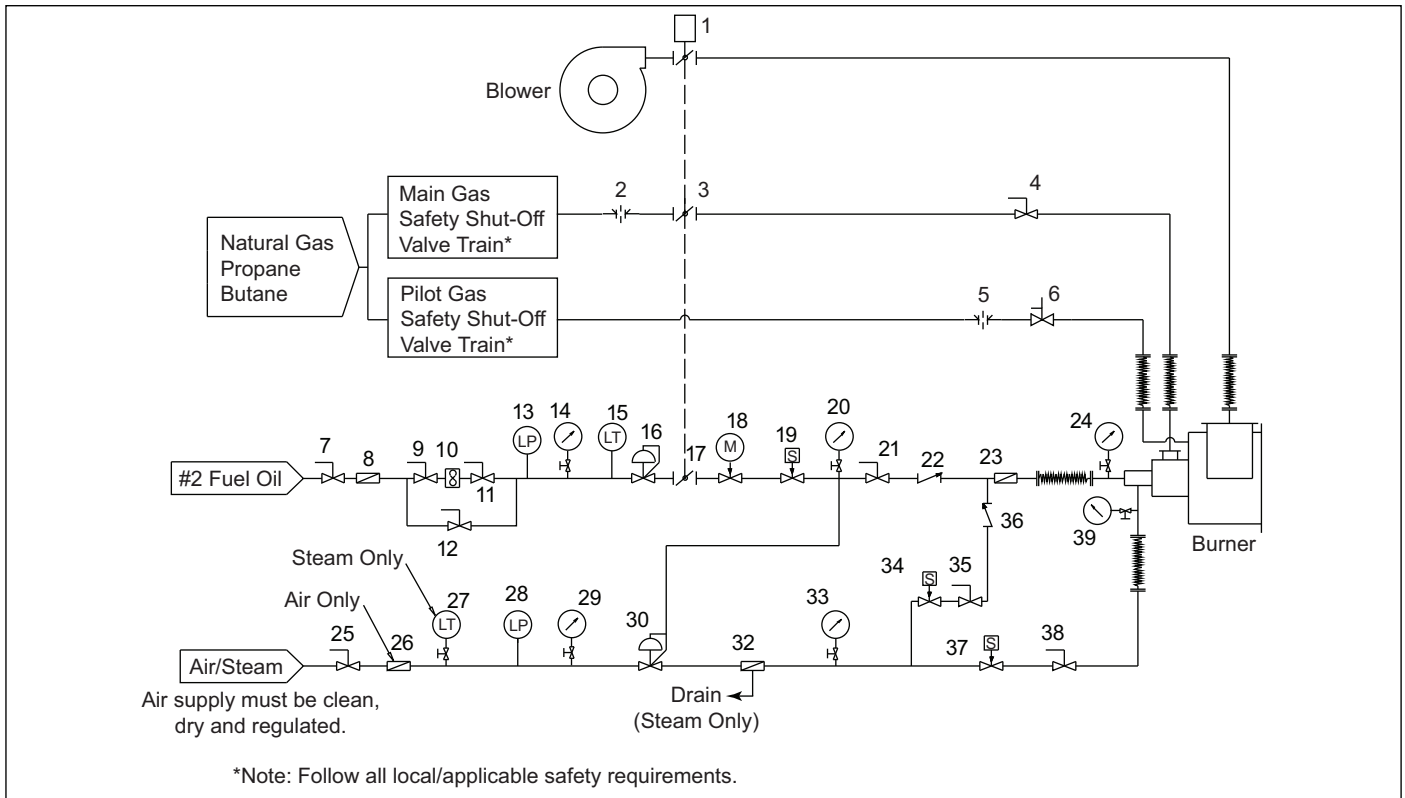
Figure 3.6 - Schematic for Natural Gas, Propane, Butane & #2 Fuel Oil
